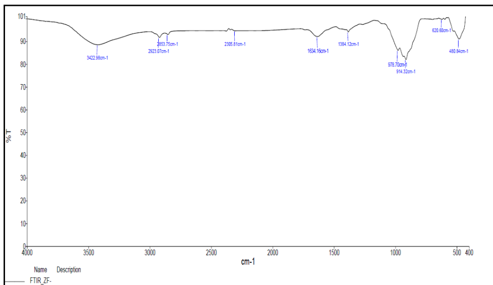
Fig-3: FTIR Pattern for CeNO 3 and Green Extract NPs
