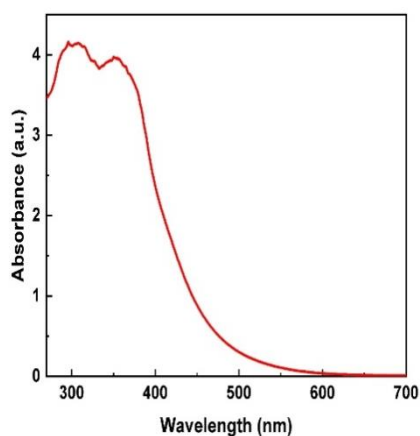
Fig.1: UV- Vis Spectrum of carbon dots
