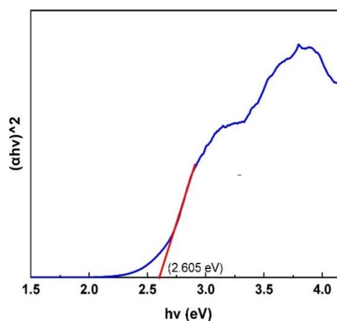
Fig.2: Extrapolated plot of (\alpha hv)^2 vs. hv obtained from the absorption spectra
