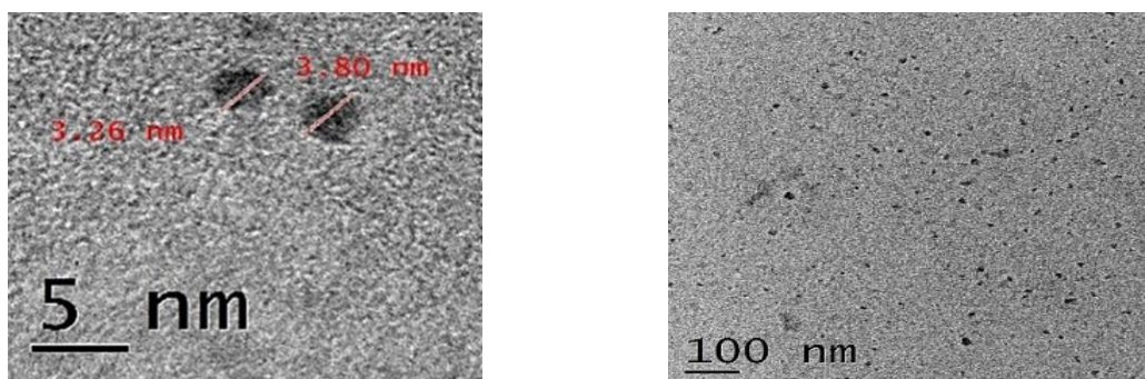
Fig. 5: High resolution TEM image of Carbon Dots at 5 nm and 100 nm magnifications respectively
