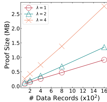
Fig. 3. Storage cost of cryptographic proofs
