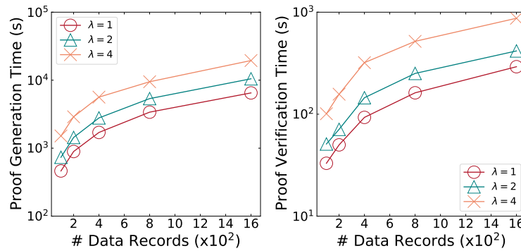
Fig. 4. CPU time for proof generation Fig. 5. CPU time for proof verification
