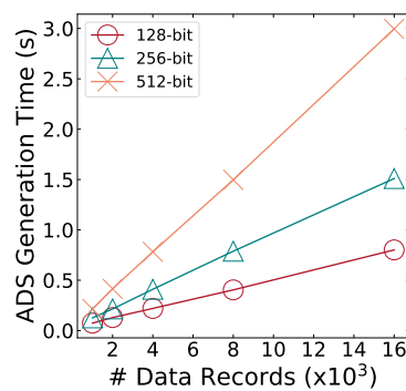
Fig. 2. Time required for ADS construction
