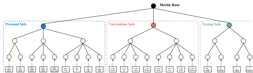
Fig. 1. ADS Construction Example for Health Monitoring Record
