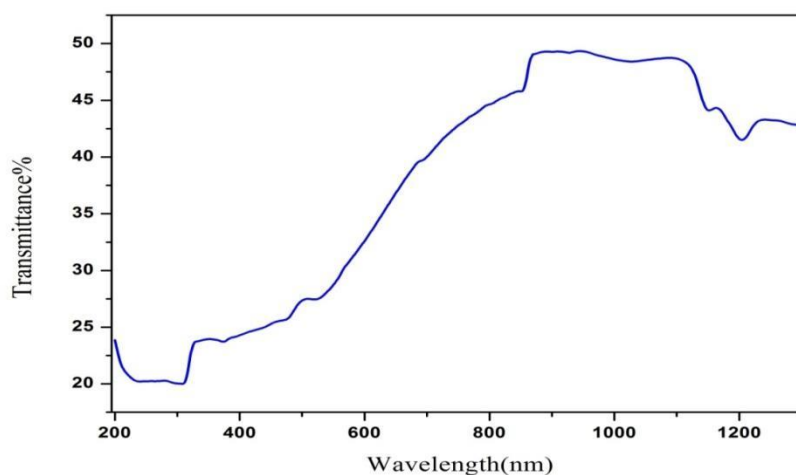
Fig 5: Transmittance spectrum of LALMA single crystal
